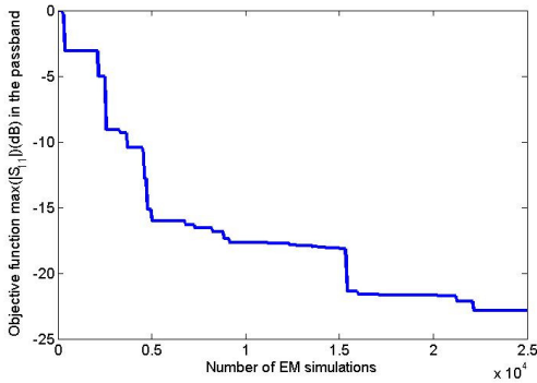
Figure 7. DE convergence trend for example 1.
