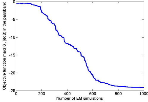
Figure 6. SMEAFO convergence trend for example 1 (average of 10 runs).
