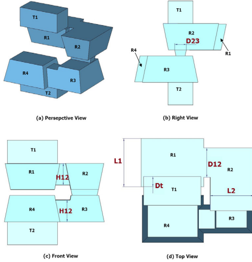
Figure 4. Waveguide filter: T1, input test port, T2: output test port, R1-R4: resonators.
