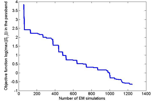
Figure 10. SMEAFO convergence trend for example 2.
