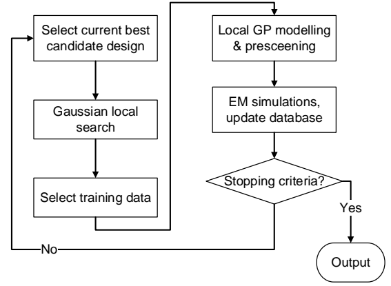
Figure 3. The flow diagram of the exploitation phase.
