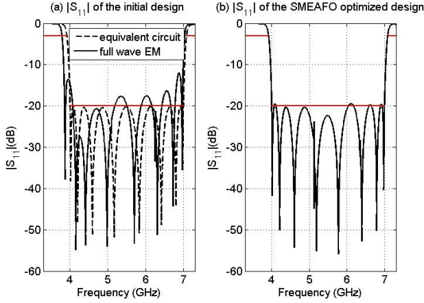
Figure 9. Response of the microstrip filter.
