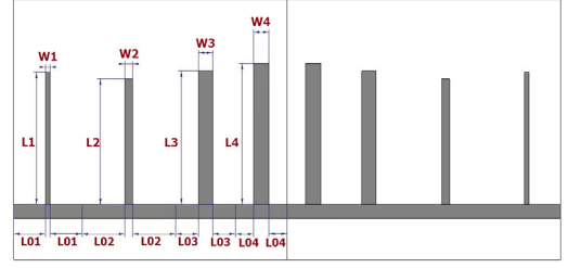
Figure 8. Microstrip filter: front view.
