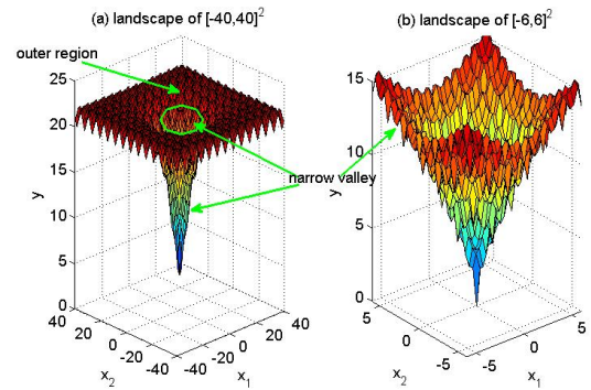
Figure 1. An illustrative figure of filter design landscape: the Ackley function [21] is used.
