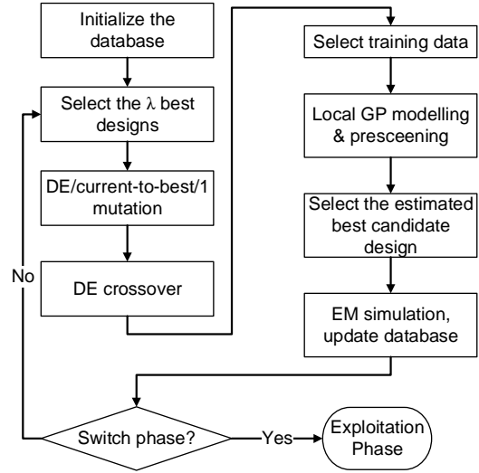
Figure 2. The flow diagram of the exploration phase.
