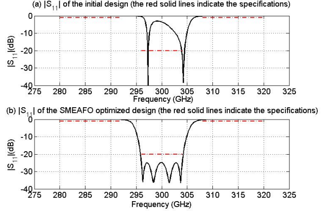
Figure 5. Response of the waveguide filter.
