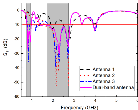
FIGURE 5. The reflection coefficient of the four reference antennas.
