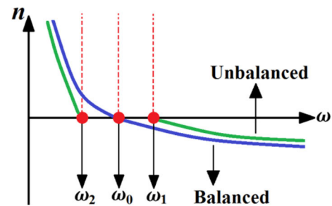
FIGURE 4. Typical index of refraction diagrams for the balanced- and unbalanced-CRLH TLs in blue and green, respectively.
