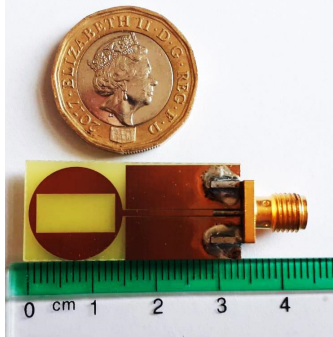
Figure 3. The microwave imaging antenna (example 2).
