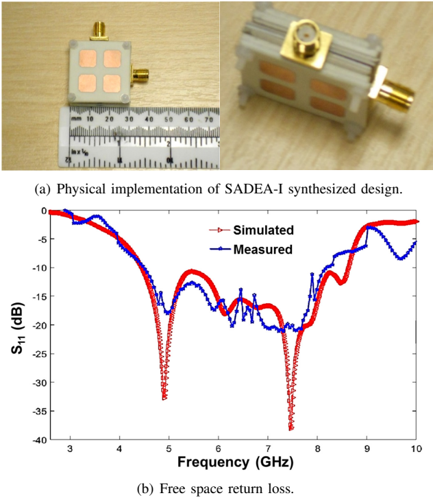
Figure 2. The multilayered compact MIMO antenna array (example 1).
