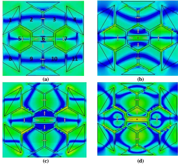
Fig. 2. Electric field distributions of the proposed MTS antenna at four resonant frequencies in the higher frequency band, at (a) 5.0, (b) 5.8, (c) 7.0 and (d) 7.6 GHz.
