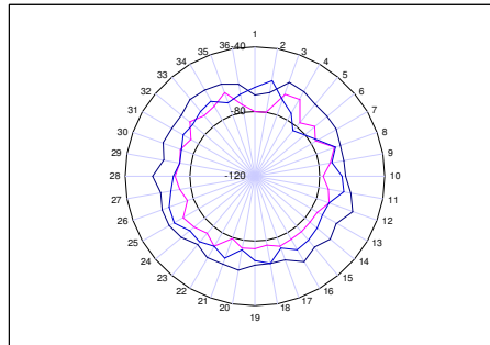
Figure 5: Measured signal strength around base station
