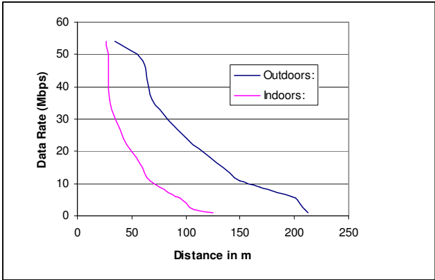
Figure 3: Graph of Maximum Connection Distances
