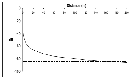
Figure 9: Distance versus signal strength
