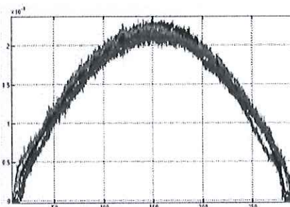
Fig. 13 Uniformity of removal over three runs
