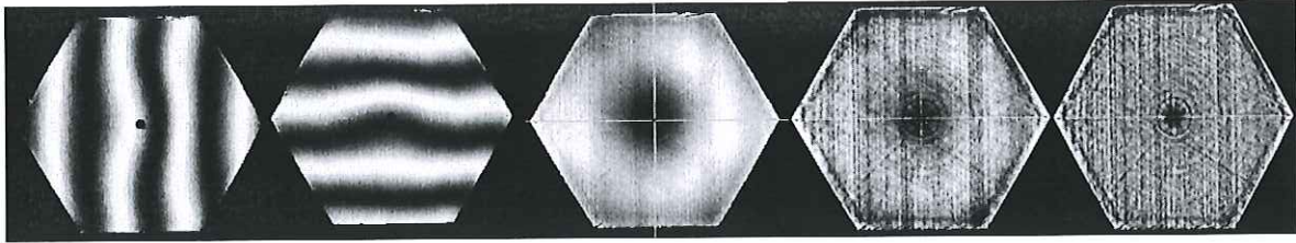
Fig. 4 X and Y synthetic interferograms for MSS
